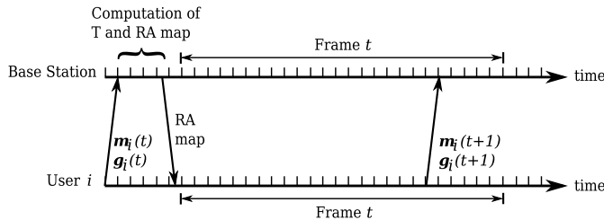
Fig. 1. Resource allocation timeline.
