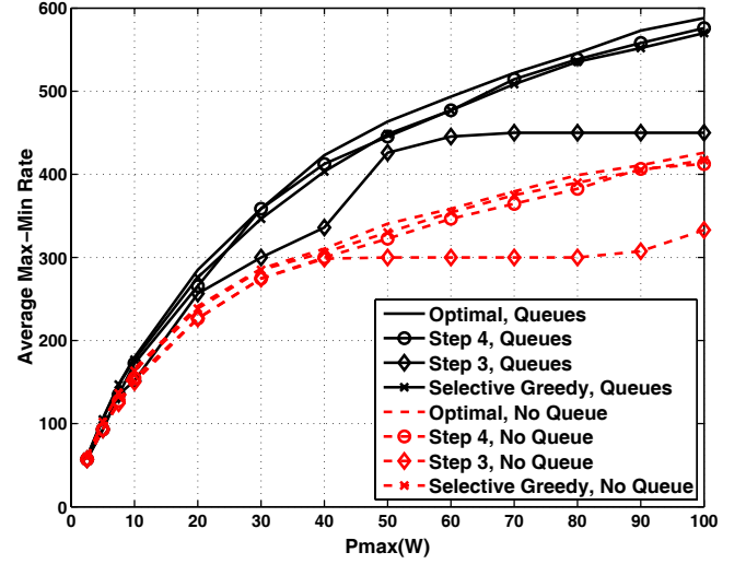
Fig. 6. Average max-min per frame rate of the optimal solution and heuristics versus \bar{P}_{\max} for F = 1 , (M, N, N_p) = (120, 40, 0) .
