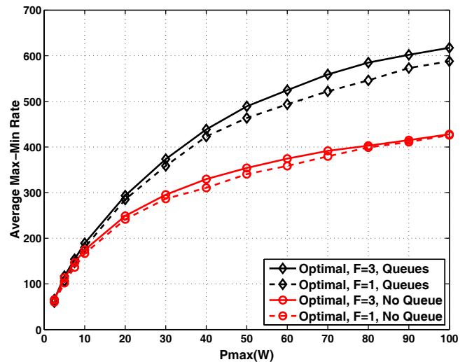
Fig. 3. Average per frame max-min rate of the optimal solution versus \bar{P}_{\max} for F = 1, 3 , (M, N, N_p) = (120, 40, 0) .
