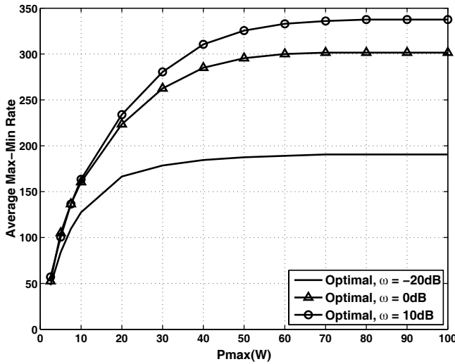
Fig. 5. Average max-min per frame rate of the optimal solution versus \bar{P}_{\max} for F = 1 , (M, N, N_p) = (120, 40, 50) for several critical interference threshold \omega choices.
