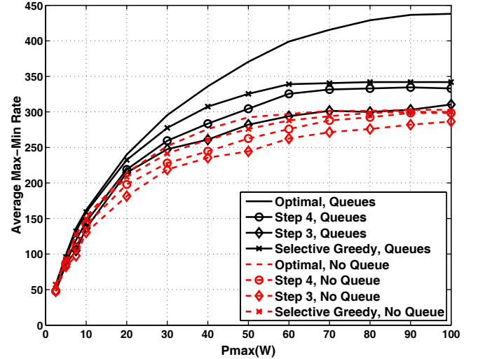
Fig. 7. Average max-min per frame rate of the optimal solution and heuristics versus \bar{P}_{\max} for F = 1 , (M, N, N_p) = (120, 40, 60) .
