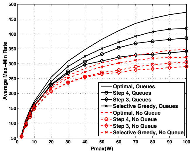
Fig. 8. Average max-min per frame rate of the optimal solution and heuristics versus \bar{P}_{\max} for F = 3 , (M, N, N_p) = (120, 40, 60) .
