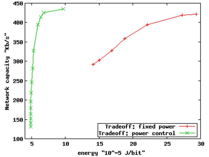
Fig. 8. The energy and capacity tradeoff: fixed power vs continuous power control (random network and multi-rate transmission).
