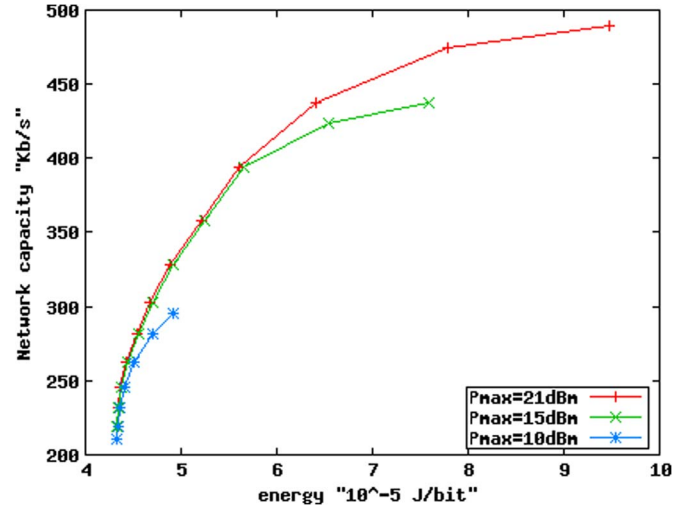
Fig. 6. Impact of maximum power transmission on energy-capacity tradeoff: random network with MCS4.
