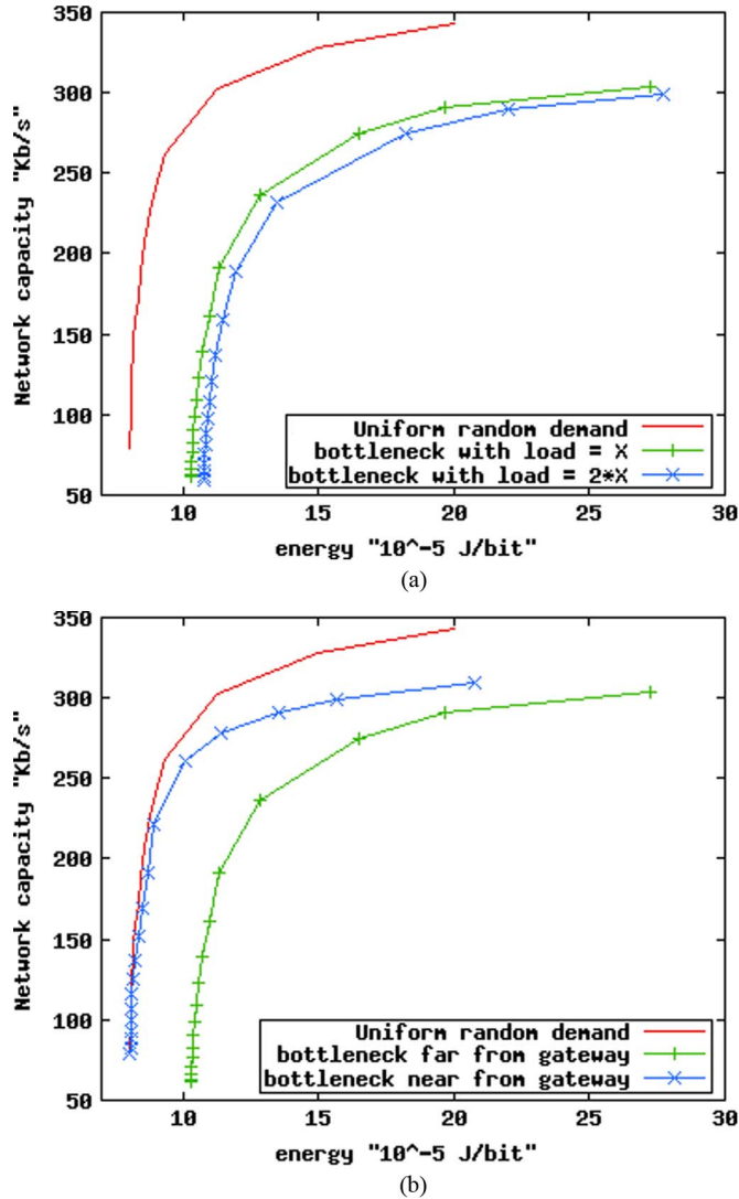
Fig. 11. Impact of bottleneck on energy-capacity tradeoff with MCS3 and continuous power control. (a) Impact of the magnitude of the bottleneck on the energy-capacity tradeoff. (b) Impact of the distance between the bottleneck and the gateway on the energy-capacity tradeoff.
