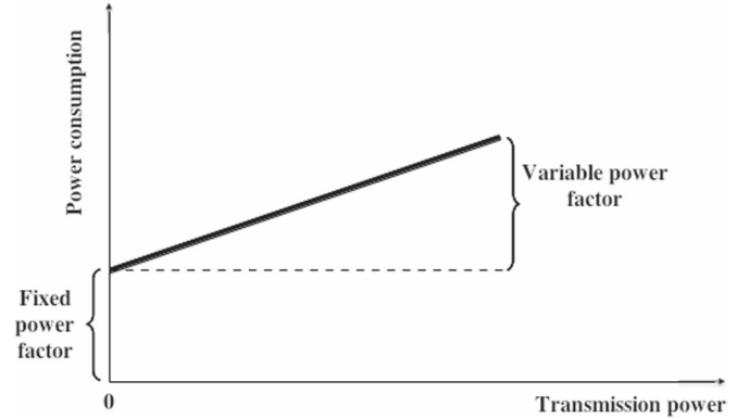
Fig. 2. Illustration of the power consumption model.
