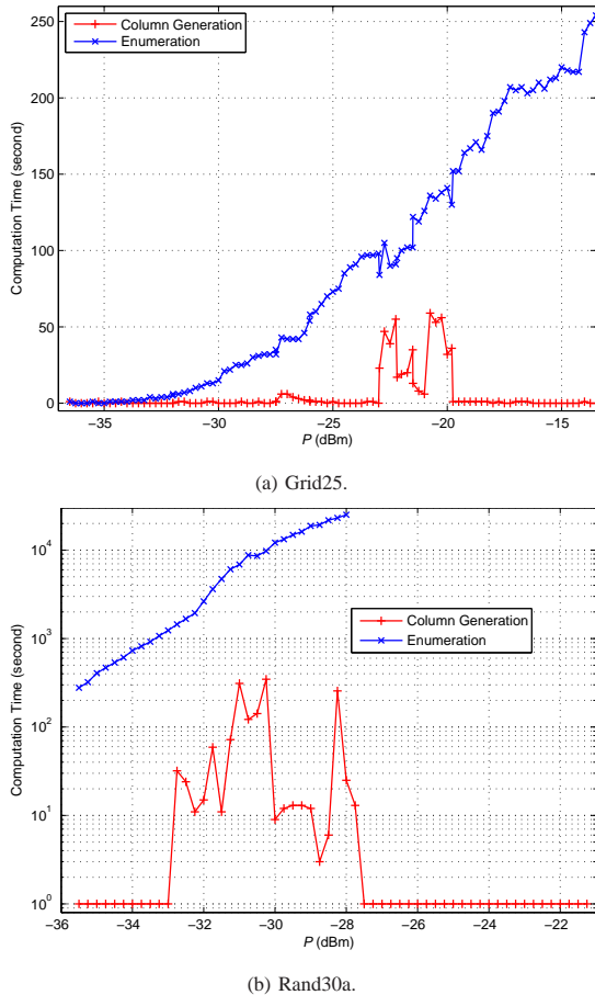
Fig. 2. Computation times for the two exact algorithms for the case with converging traffic
