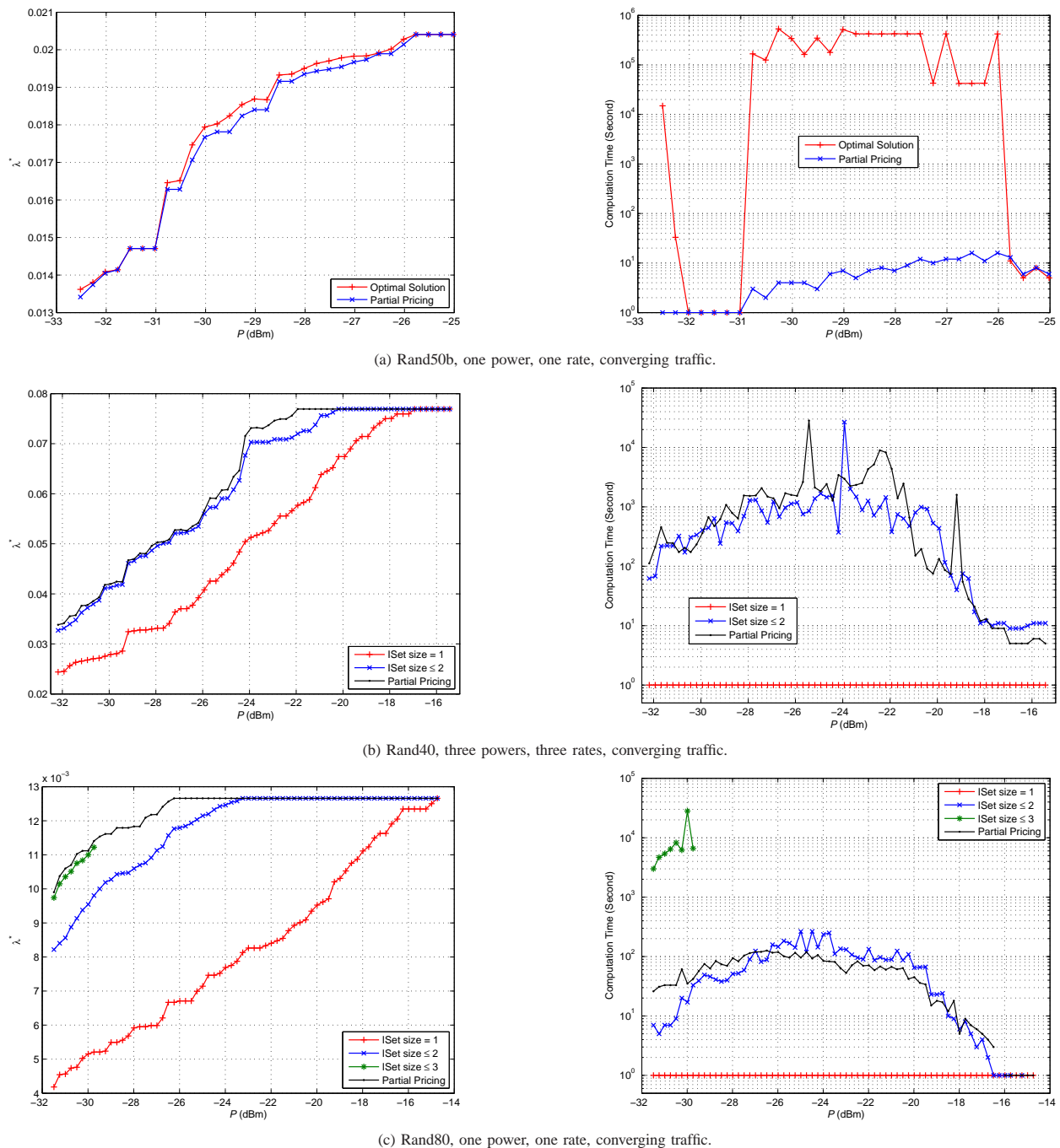
Fig. 9. Comparisons of different approximation mechanisms on different large scenarios.
