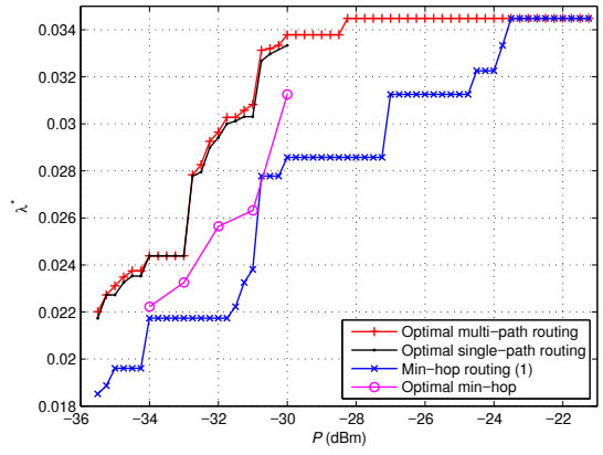
Fig. 5. Optimal multi-path and single-path routings vs. min-hop routings: Rand30a with converging traffic.
