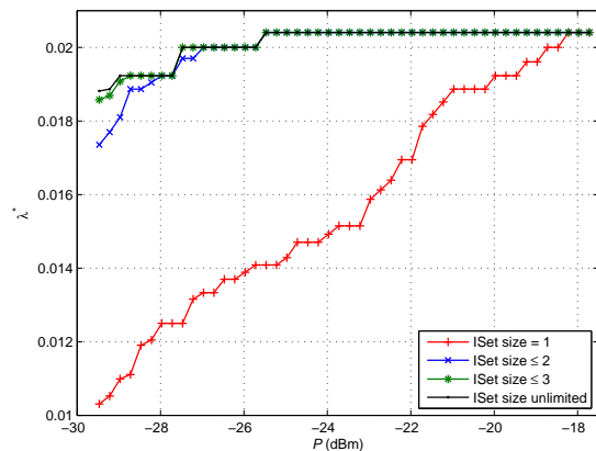
Fig. 7. Optimal max-min throughput under constraints on the maximum size of ISets: Rand50a with diverging traffic.
