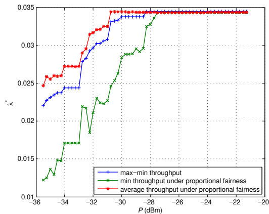
Fig. 11. Comparison of PF and max-min optimal configurations for the Rand30a network.
