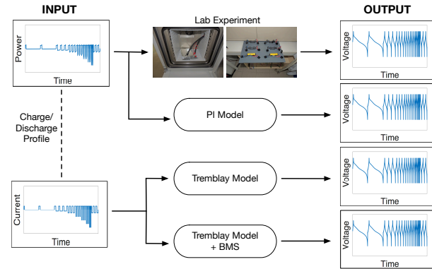
Fig. 11. Evaluation setup. Charge/discharge profiles were tested on real cells, our PI model, and two implementations of the TD model.
