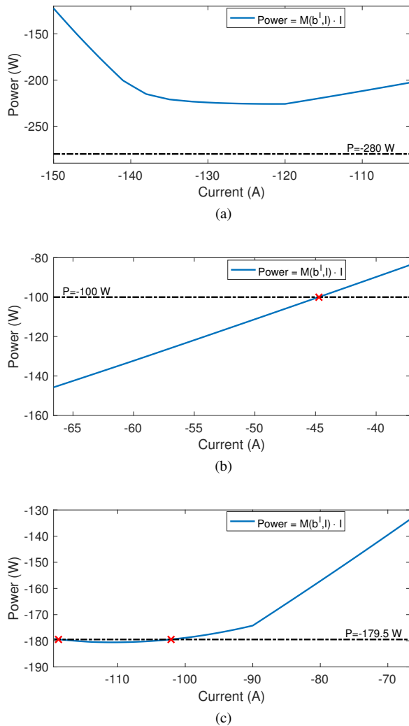
Fig. 3. Three cases: No intersection (a), one intersection (b), and multiple intersections (c). A red cross indicates an intersection.
