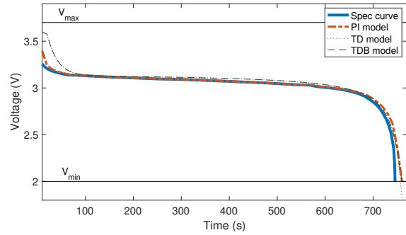
Fig. 8. LiFePO 4 cell discharged at 4.55 C constant current.
