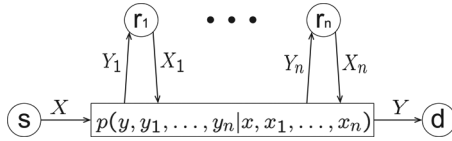
Fig. 2. Multiple-relay channel.
